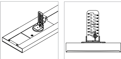
Adjustable T-Bar Clip, Small ( G1-G6 )
